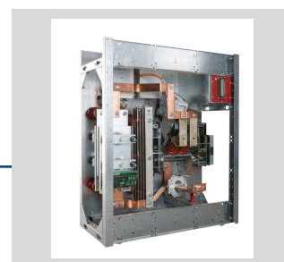
LBR-gn Withdrawable Truck Carrello estraibile LBR-gn (OPTIONAL)
